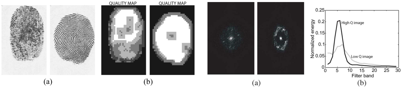
Fig. 6. Fingerprint-quality maps [panel (b)] provided by the minutia detection package of the NIST Fingerprint Image Software for two fingerprints of different quality [panel (a)].
